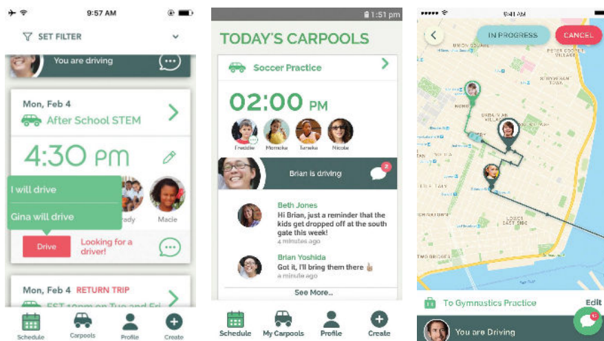
GoKid app - managing carpools
